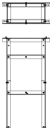
27 kV /38 kV Substation mounting bracket
