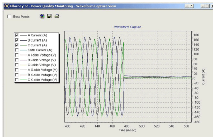
Waveform capture
