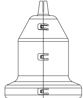
38 kV Bird guard (X Side)
