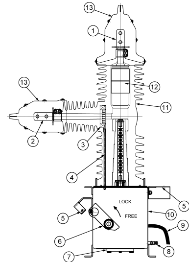
Cross section of E series 38 kV switchgear
