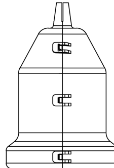
27 kV Bird guard (X Side)
