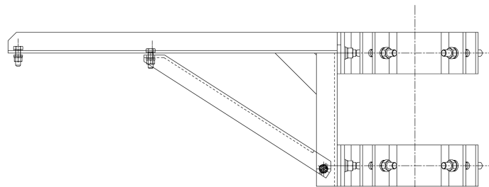
27 kV/38 kV Mounting bracket assembly (Same mounting bracket for end and center mounting)
